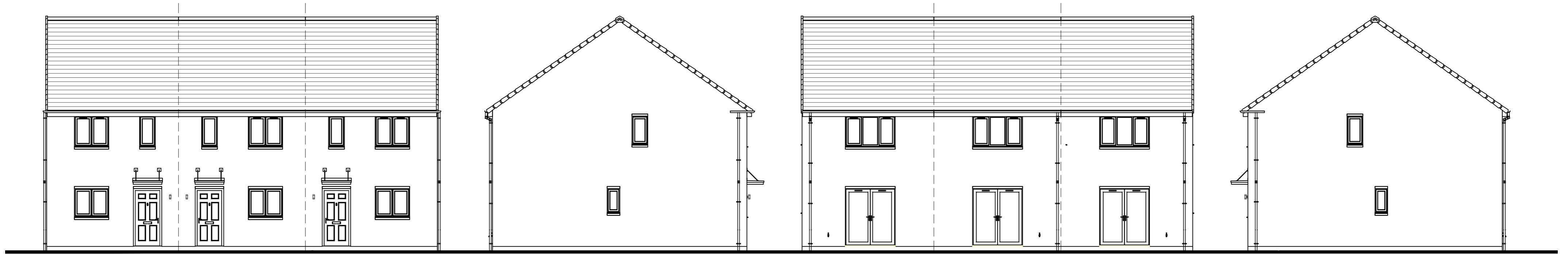
FRONT ELEVATION
