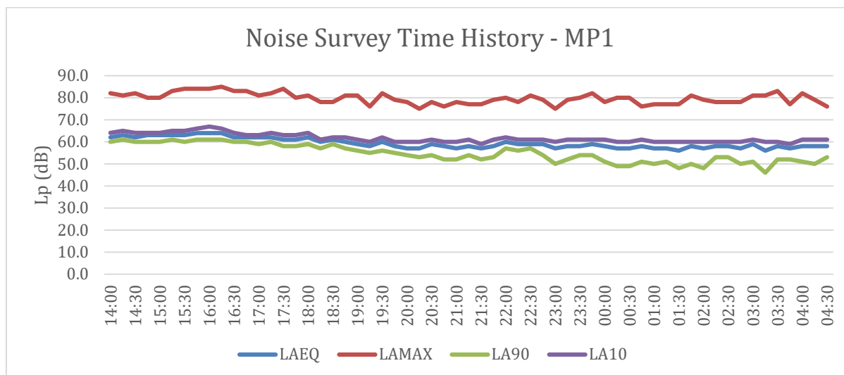
Figure 3.0 – Noise Survey Time History – MP1
