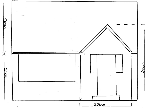
PROPOSED FRONT PORCH ELEVATION
