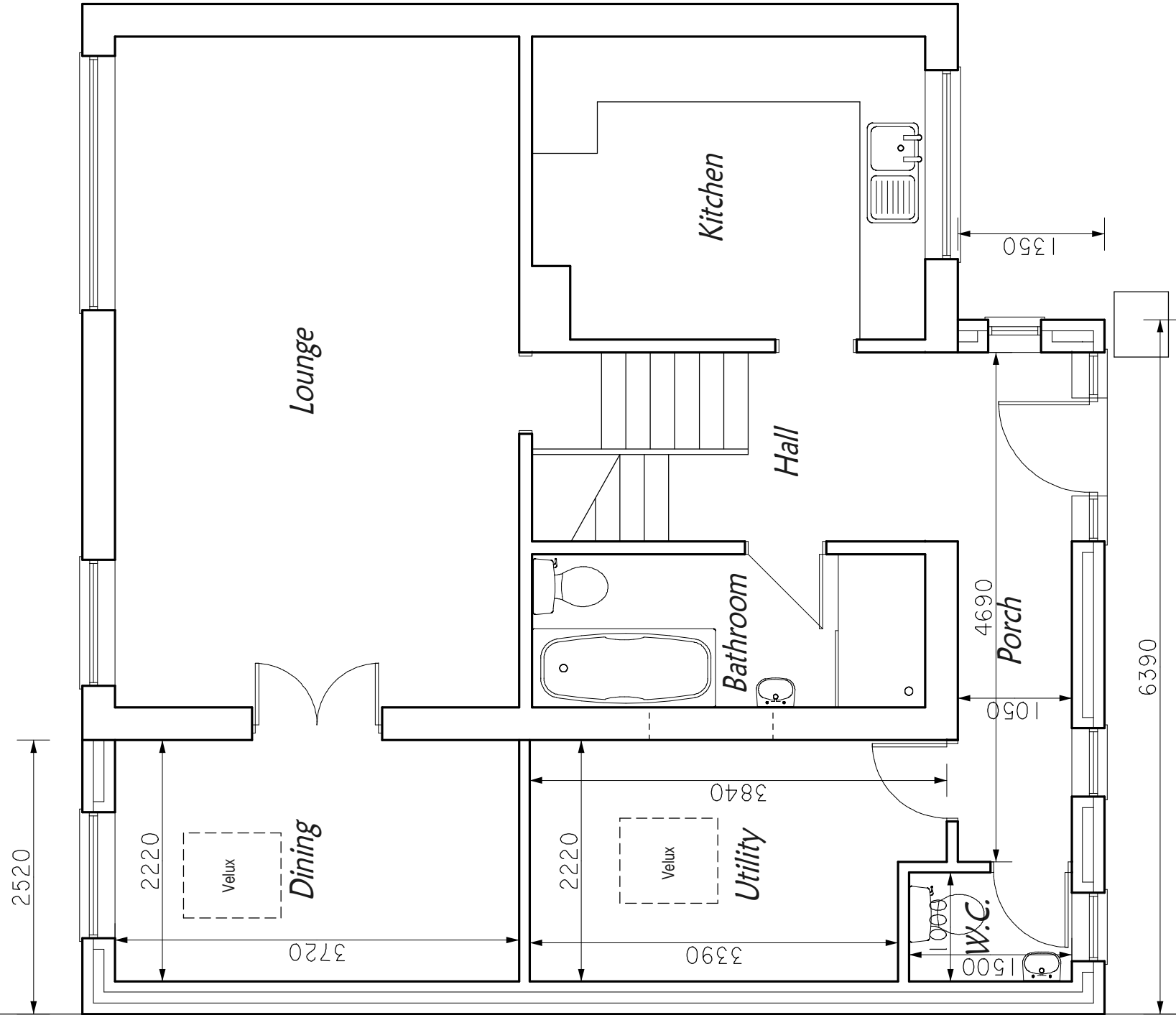
PROPOSED GROUND FLOOR LAYOUT
