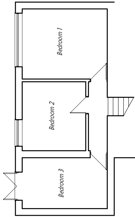
EXISTING LOWER GROUND FLOOR
