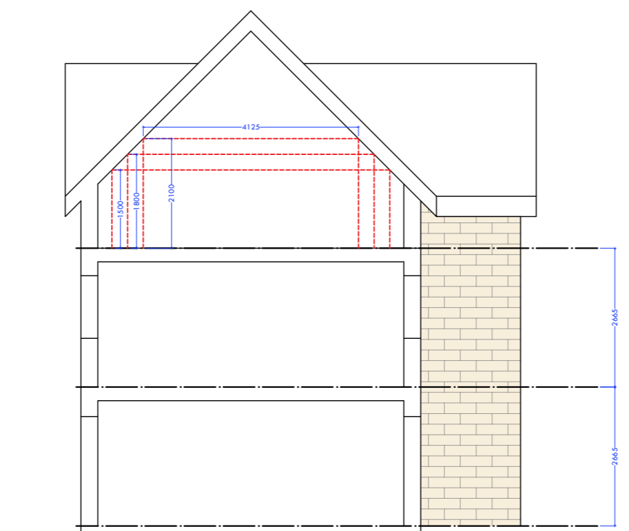
Draft Section
