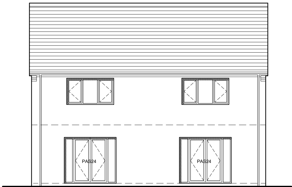
Rear Elevation
