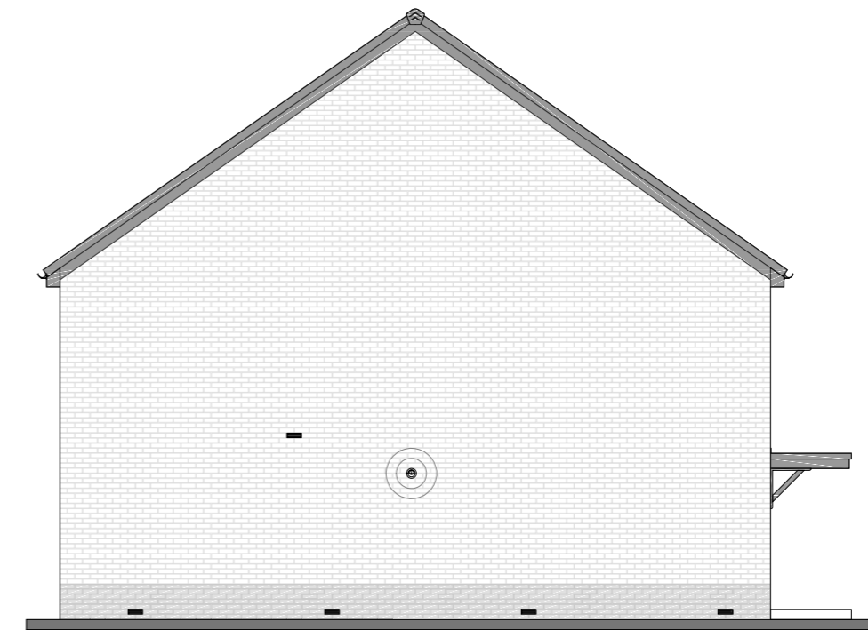
LEFT ELEVATION
