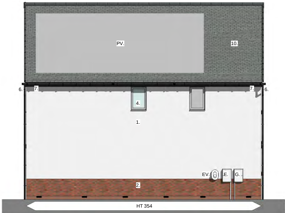
Side Elevation 1 : 100
