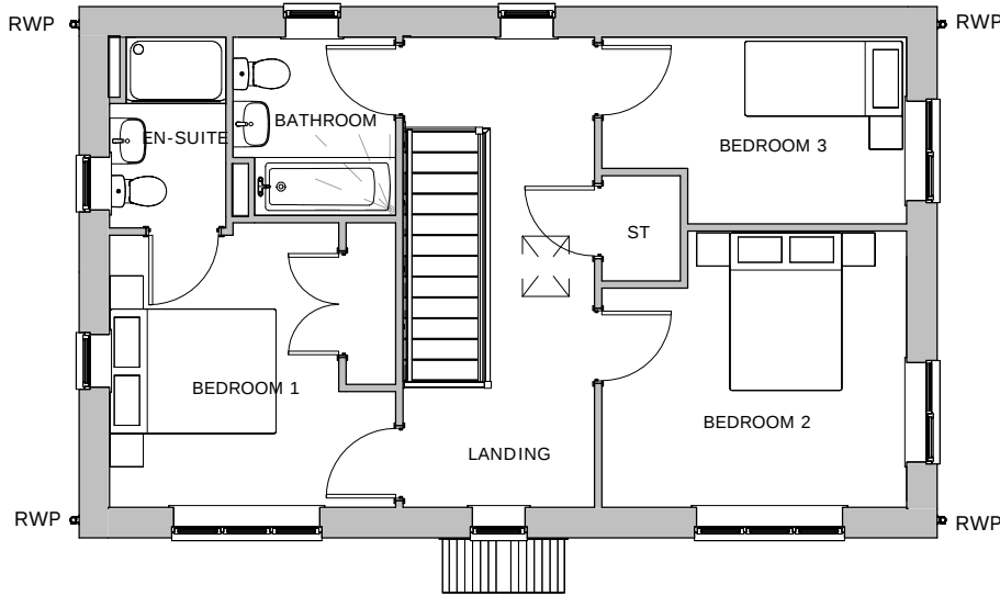
First Floor 1 : 100
