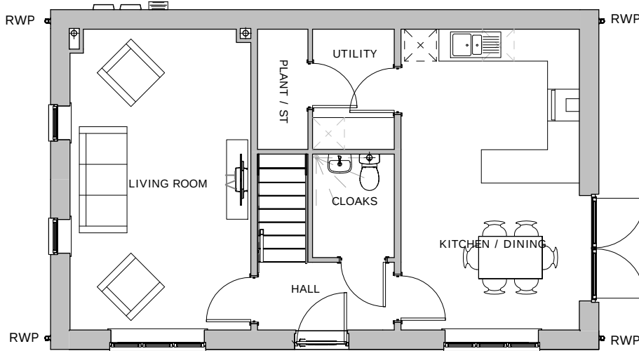
Ground Floor 1 : 100
