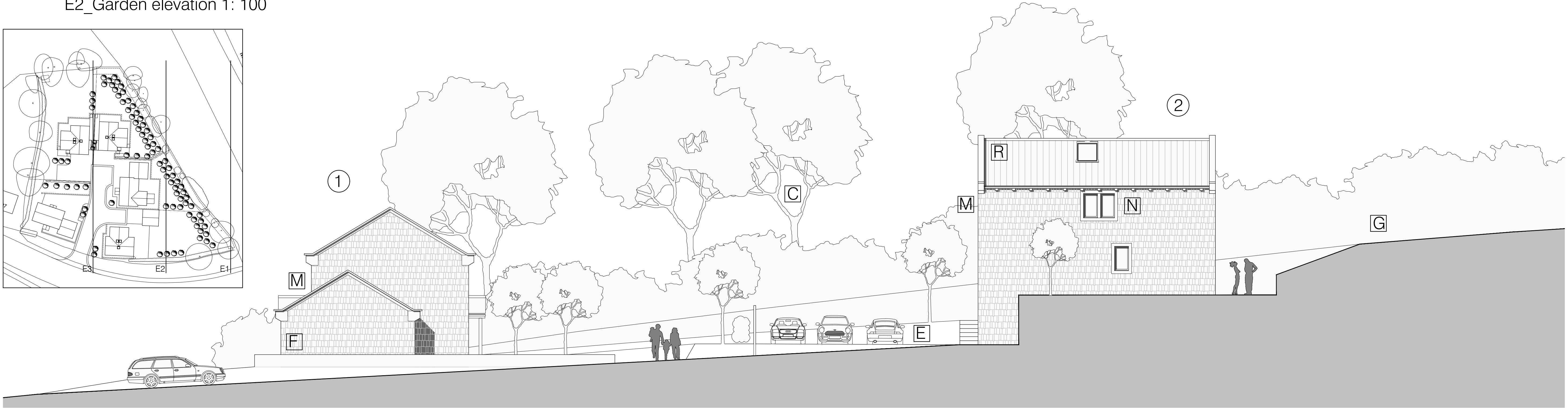
E3_Access Road elevation 1: 100
