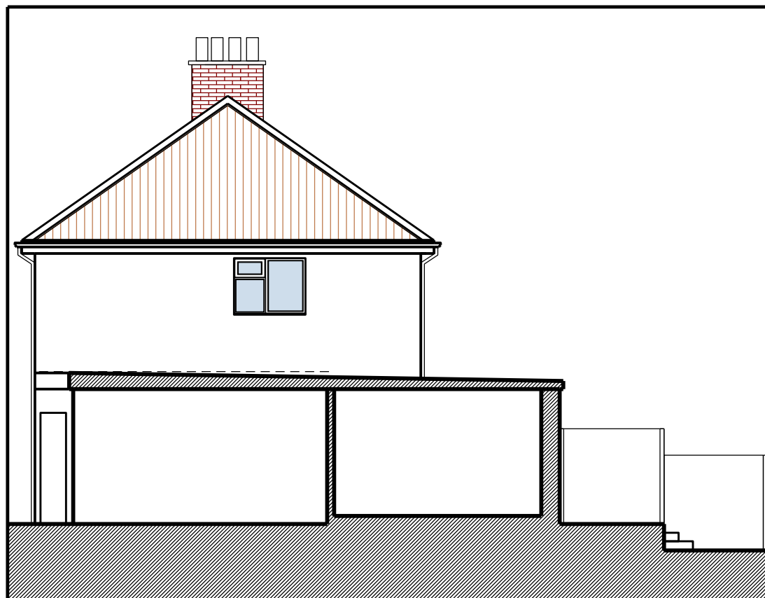
South Elevation
