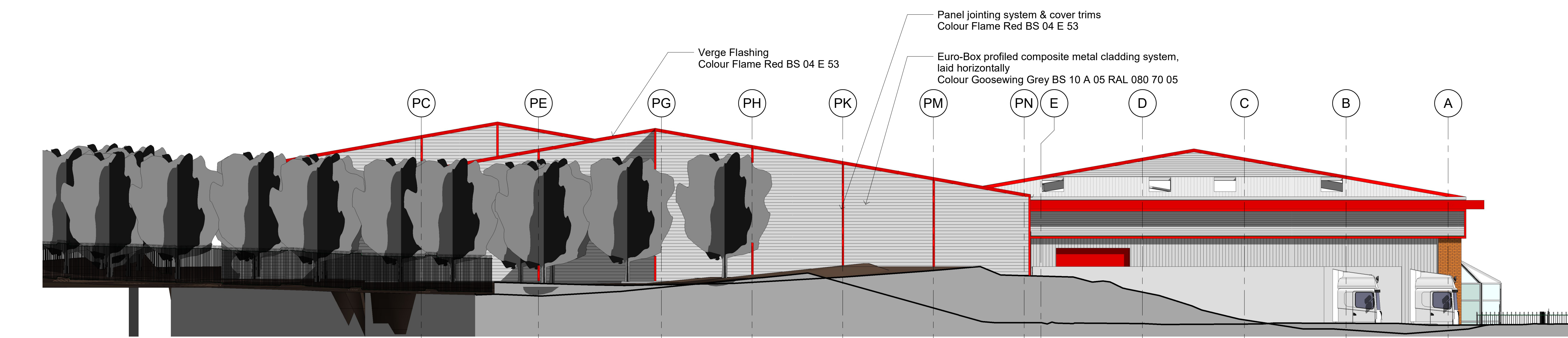
4 Elevation 4 East As Proposed 1 : 100
