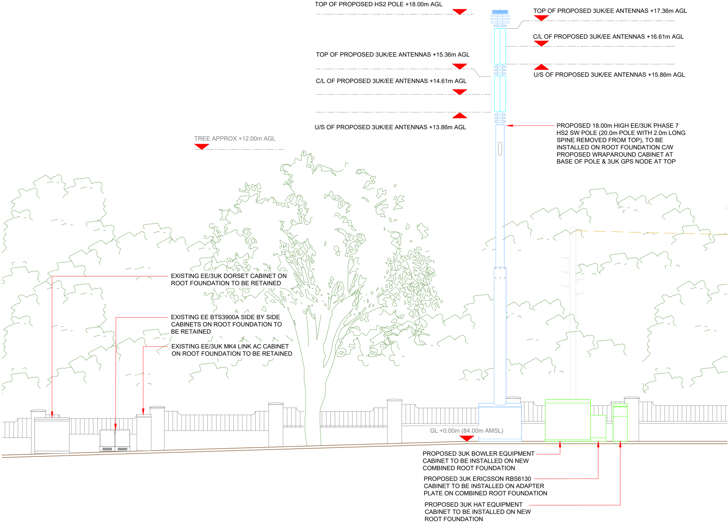
PROPOSED ELEVATION A (PLANNING)
