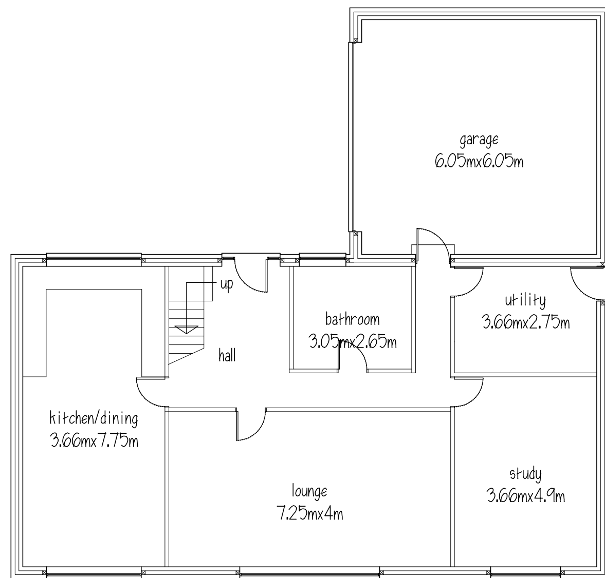
GROUND FLOOR
