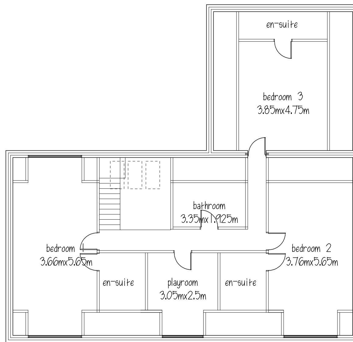
FIRST FLOOR
