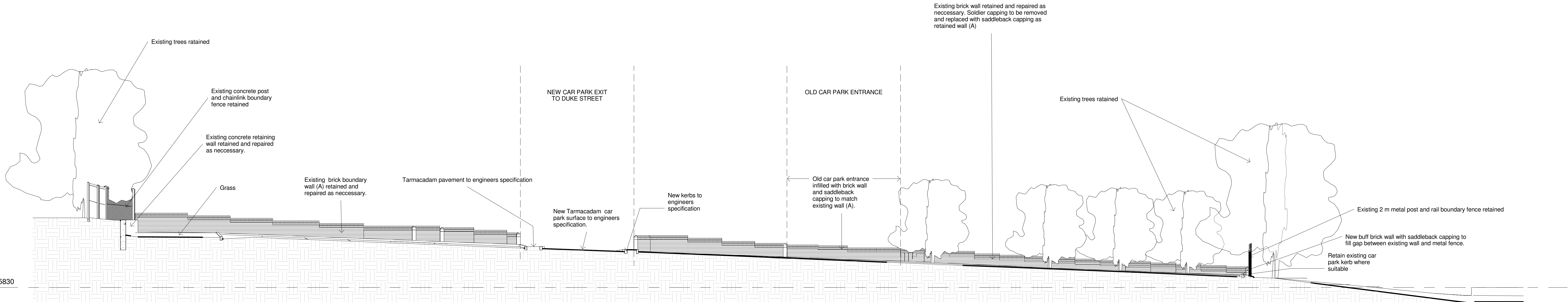
Section B As Proposed 1 : 100
