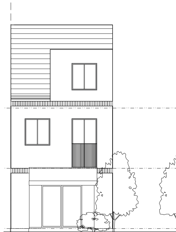
REAR ELEVATION
