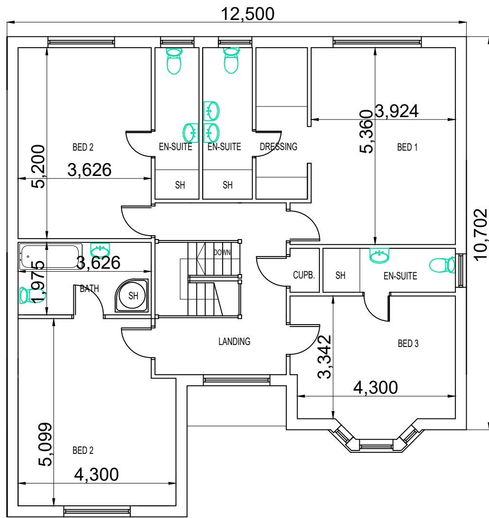
FIRST FLOOR PLAN 1:100 GROSS INTERNAL FIRST FLOOR AREA APPROX. 127 M2
