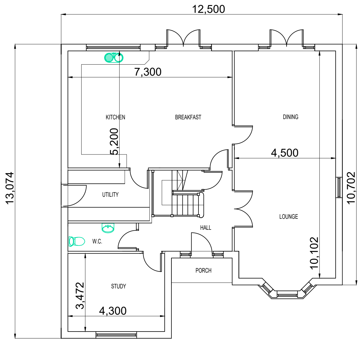
GROUND FLOOR PLAN 1:100 GROSS INTERNAL GROUND FLOOR AREA APPROX. 127 M2
