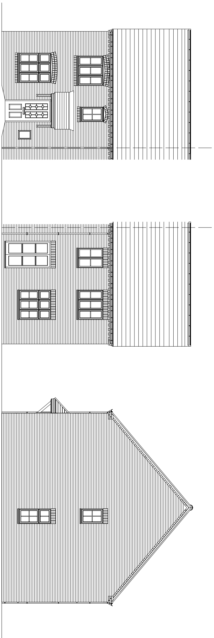
Front Elevation
