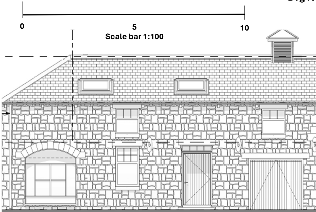
Existing front elevation – Showing Garage Door – 1:100 at A4
