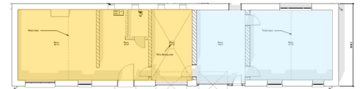
Plan view of ground and first floor - NTS
