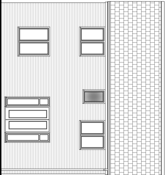
Rear Elevation
