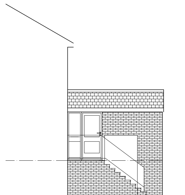
SIDE ELEVATION
