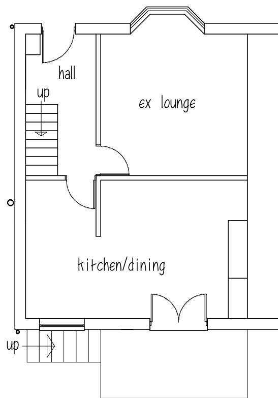
EX GROUND FLOOR
