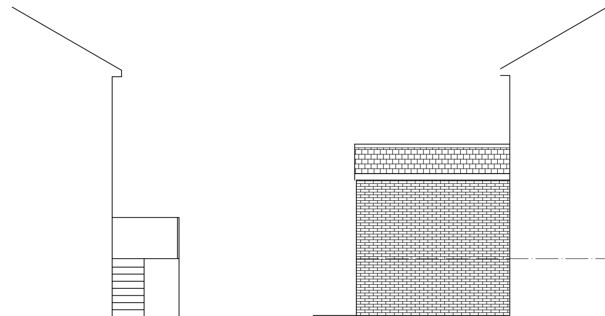
EX SIDE ELEVATION
