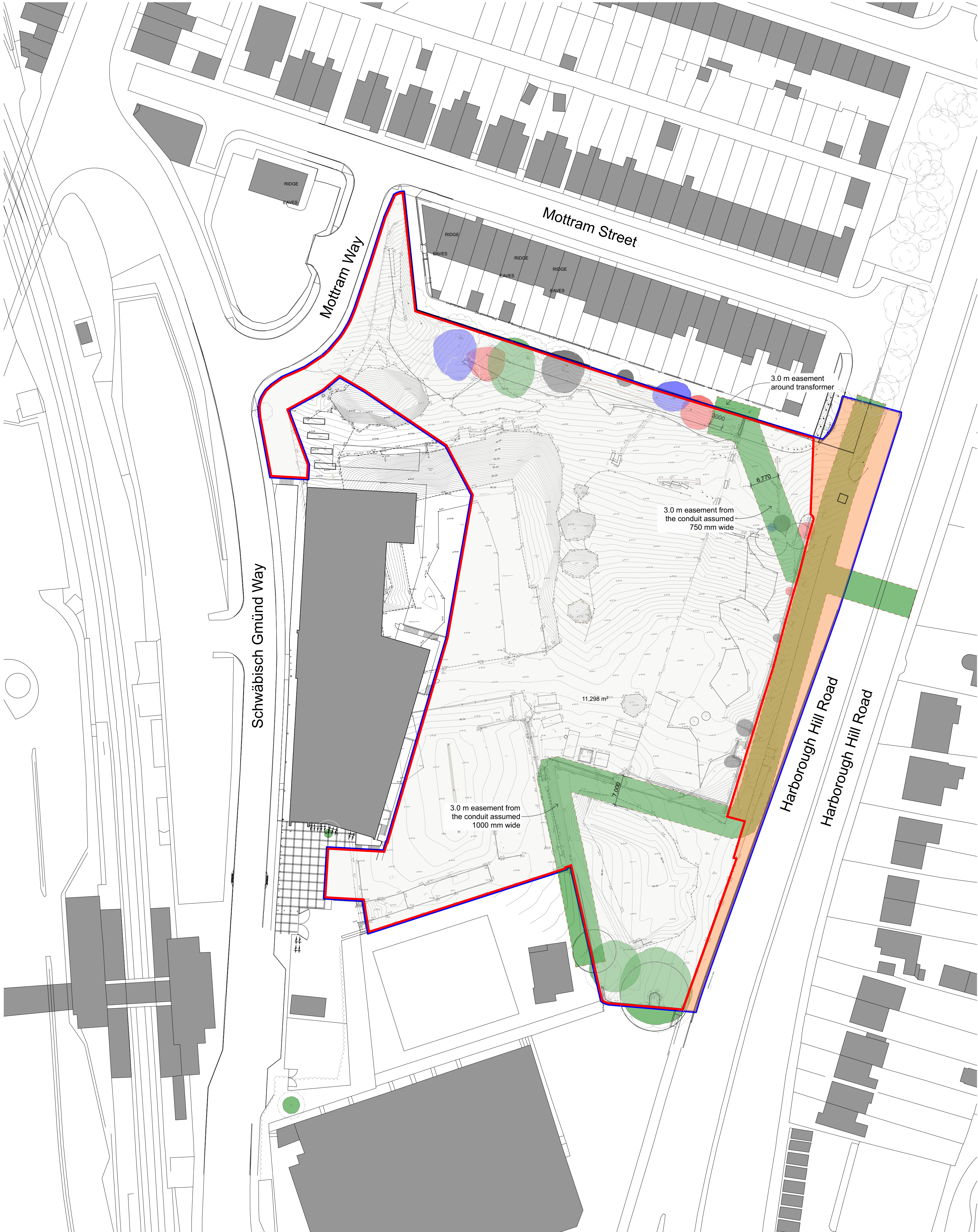
Site Boundary Plan 1:500
