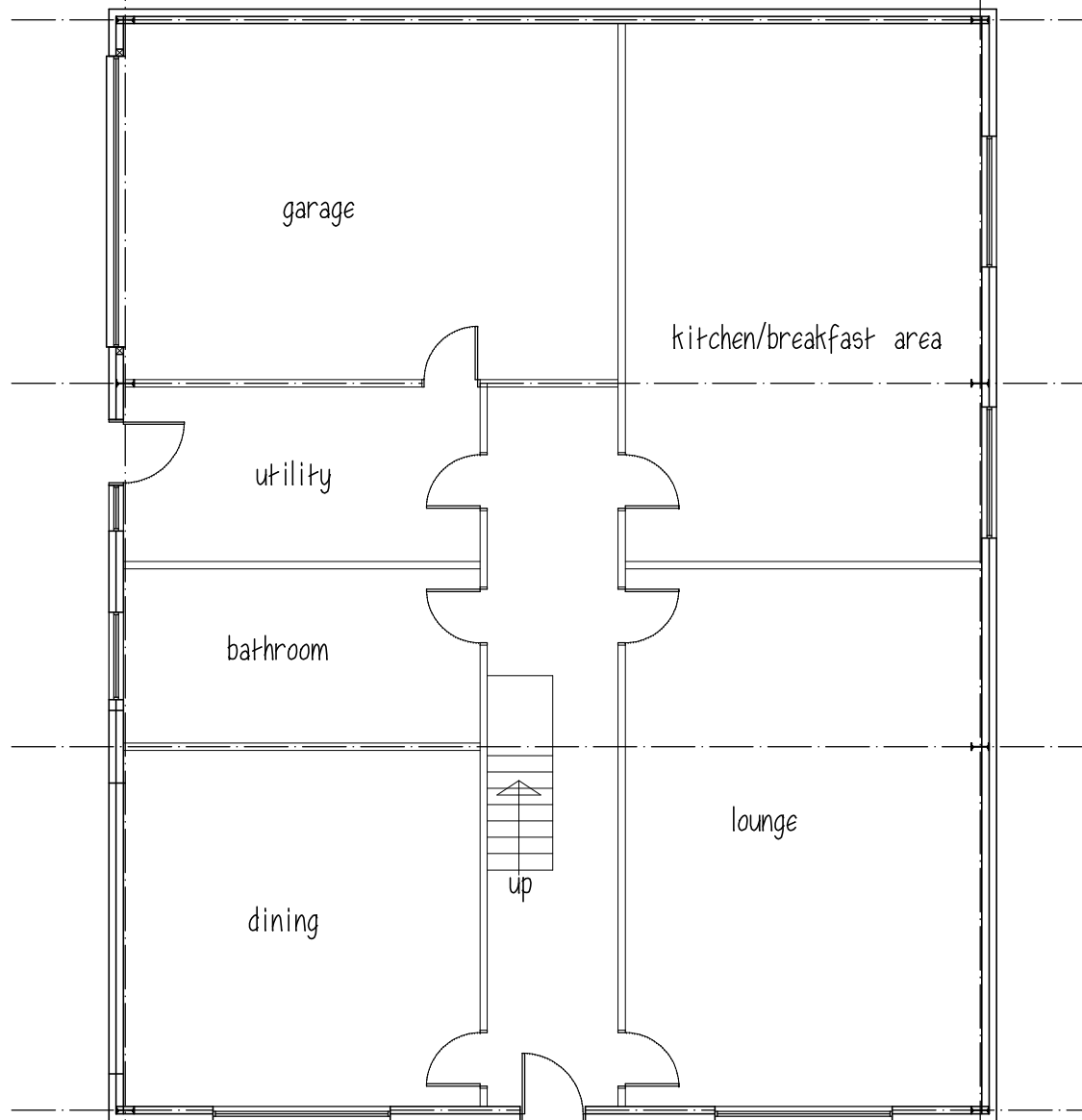
GROUND FLOOR
