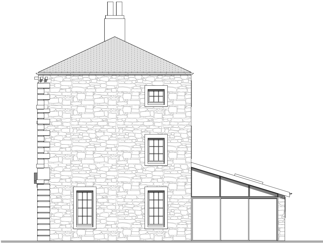
E-02 Proposed Side Elevation 1:100
