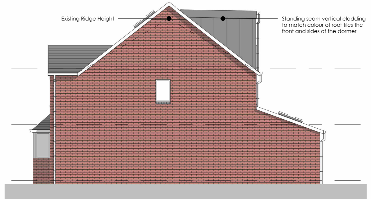
Proposed Side Elevation 02 1 : 100
