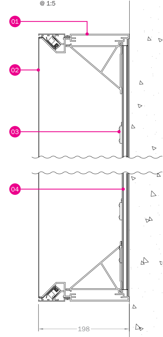
SECTION A-A @ 1:5
