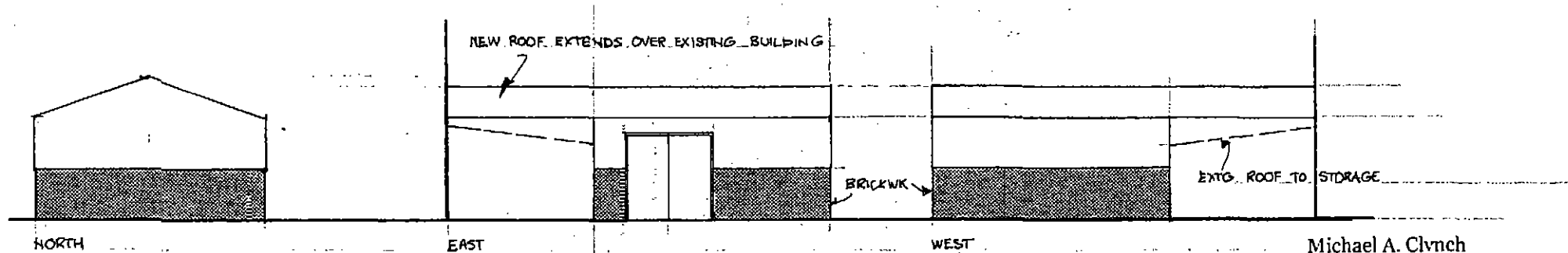
NEW GARAGE AT 17 THURLSTONE ROAD PENISTONE PLAN AND ELEVATIONS DRG A1 1:200 2/2017
