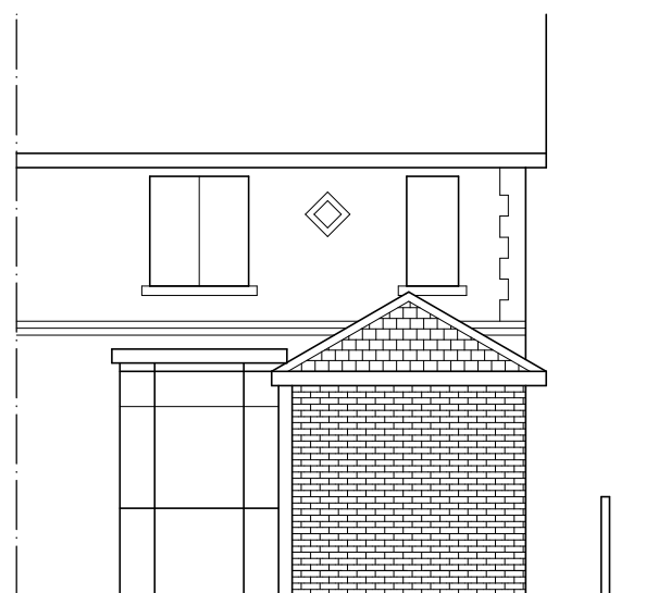
FRONT ELEVATION
