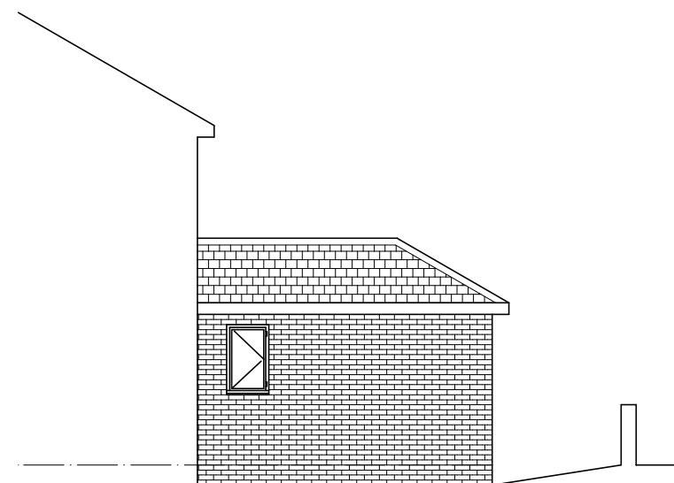
SIDE ELEVATION
