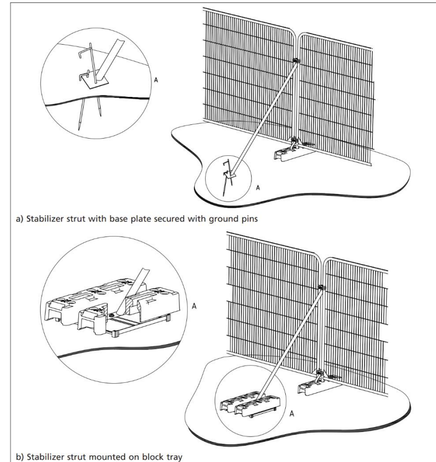
Figure 2: Alternative specification tree protection fencing. Reproduced from BS5837:2012 © BSI.
