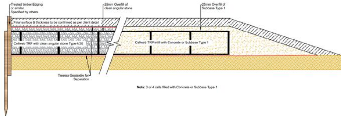
Figure 5: Example cellular confinement specification ('Cellweb TRP' Cellweb®TRP - Cellular Confinement System ). Images © Geosynthetics ( Geosynthetics - Home )
