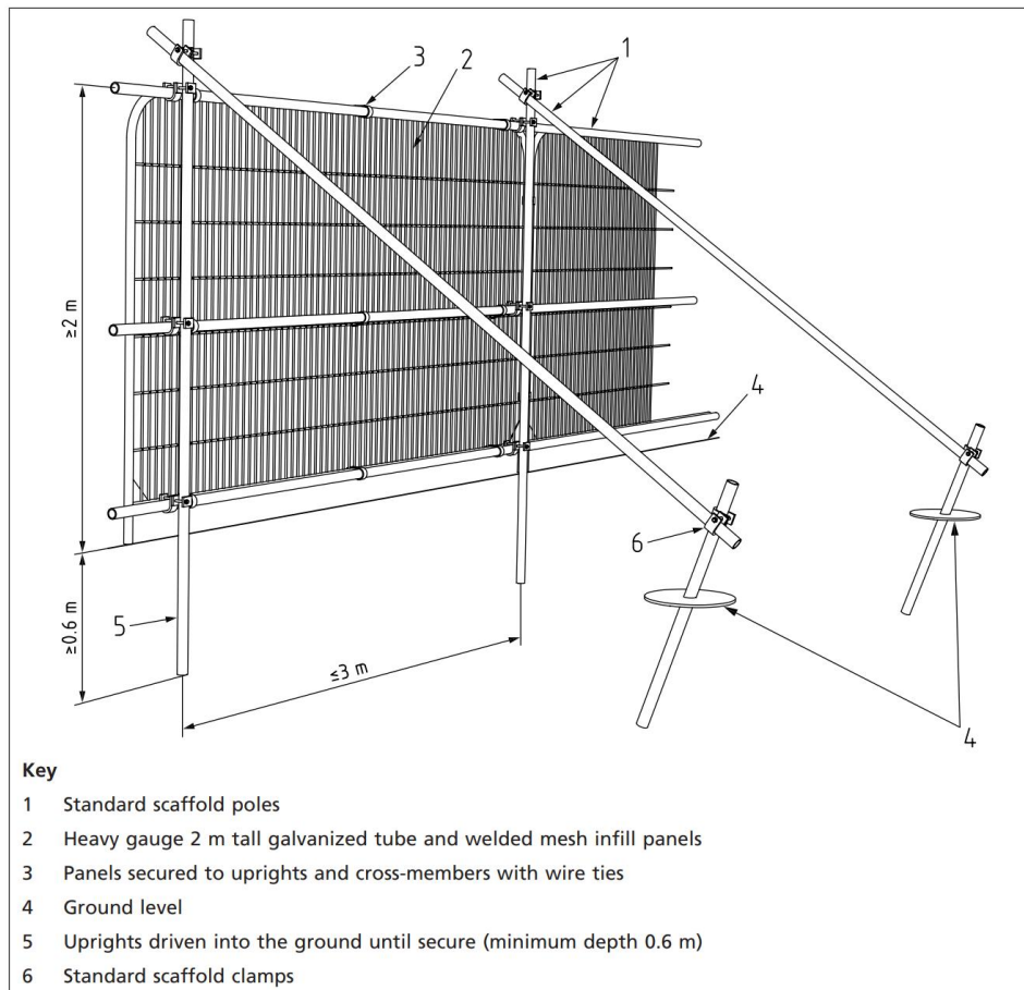
Figure 1: Default specification tree protection fencing. Reproduced from BS5837:2012 © BSI.
