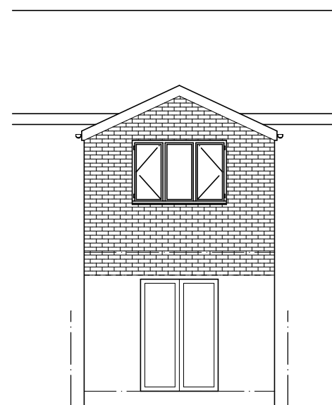
REAR ELEVATION
