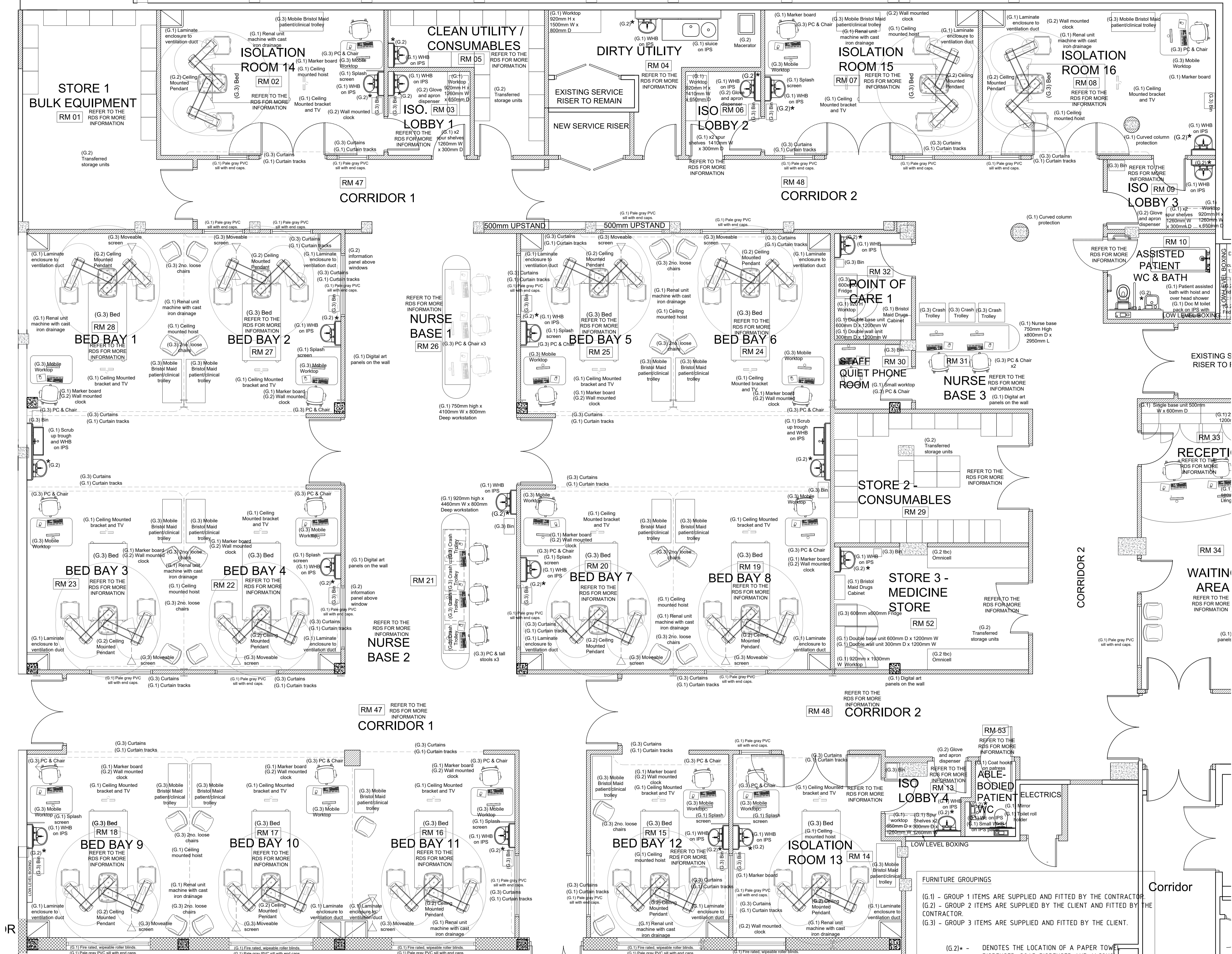
PROPOSED LOADED FURNITURE PLAN 1:100
