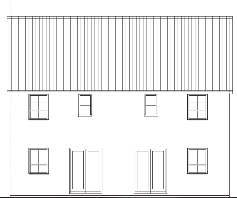
REAR ELEVATION
