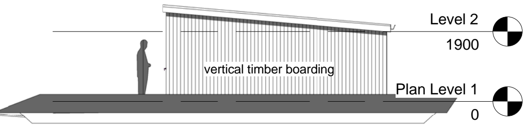
6 West Elevation 1 : 100
