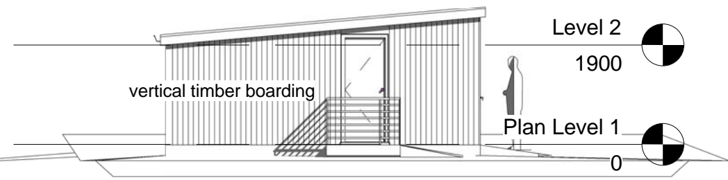
4 East Elevation 1 : 100
