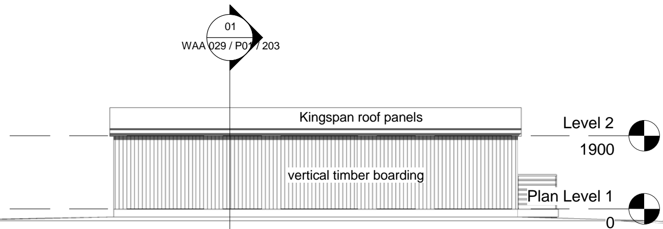
5 South Elevation 1 : 100
