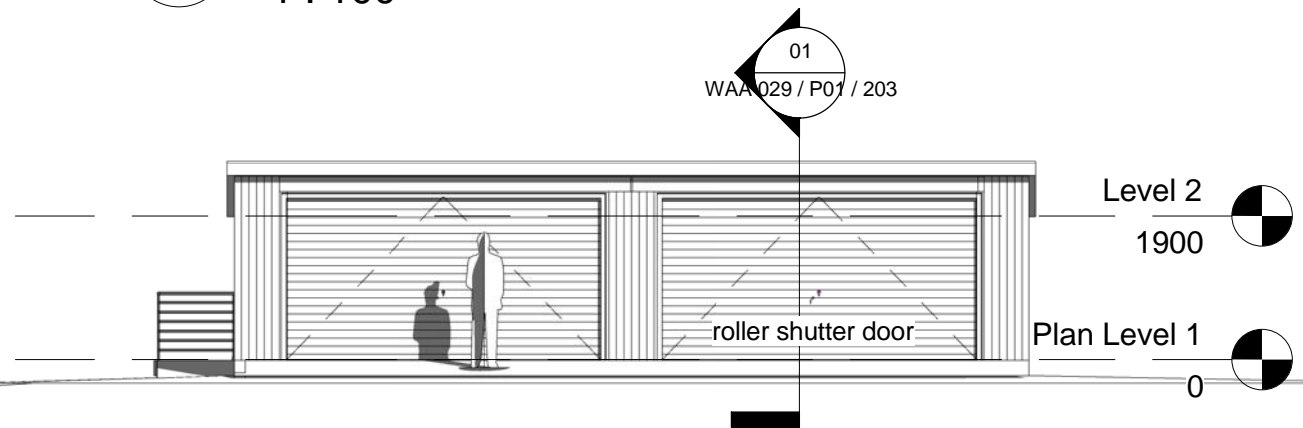
3 North Elevation 1 : 100
