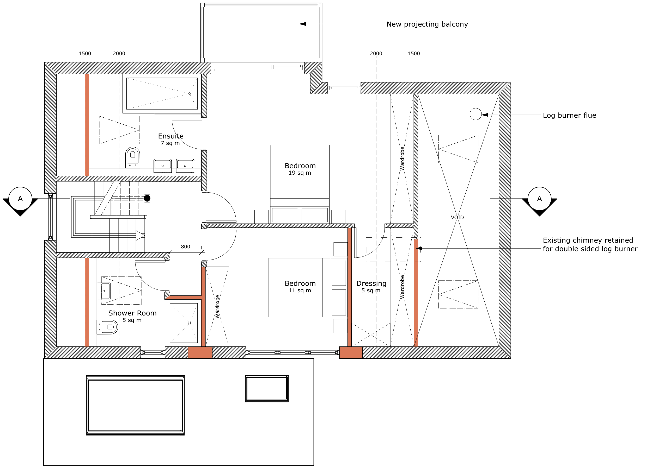
1 Proposed First Floor Plan Scale: 1:50
