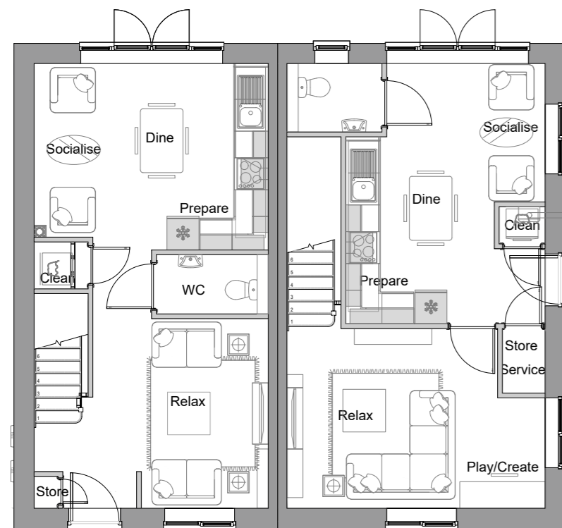
GROUND FLOOR
