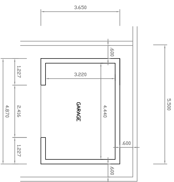
PROPOSED FLOOR LAYOUT
