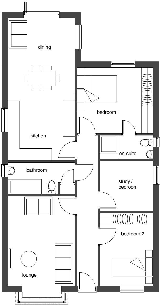
FLOOR PLAN
