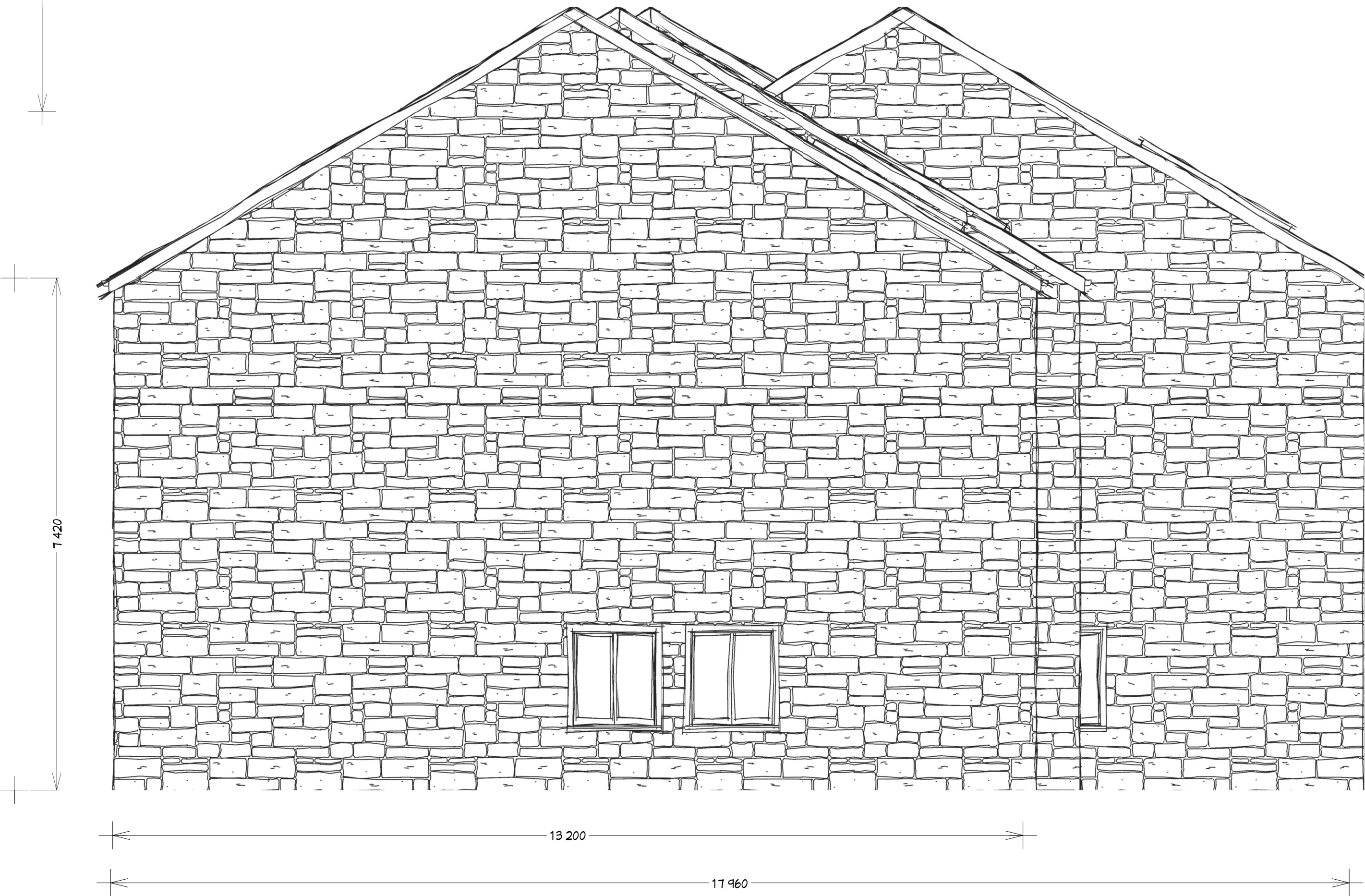
left elevation
