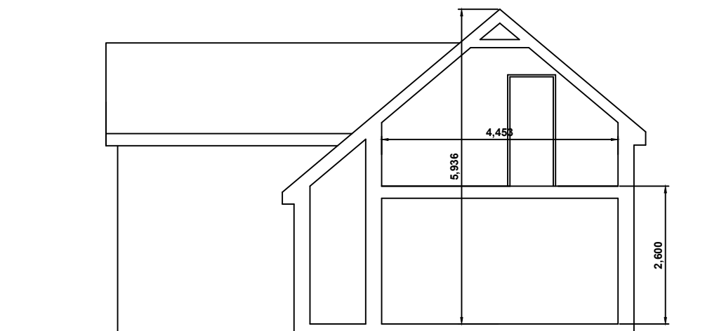
basic section
