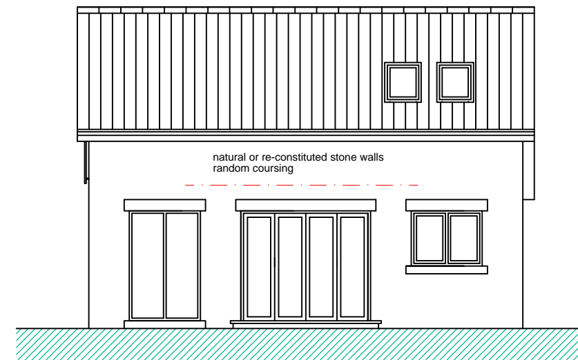
south elevation
