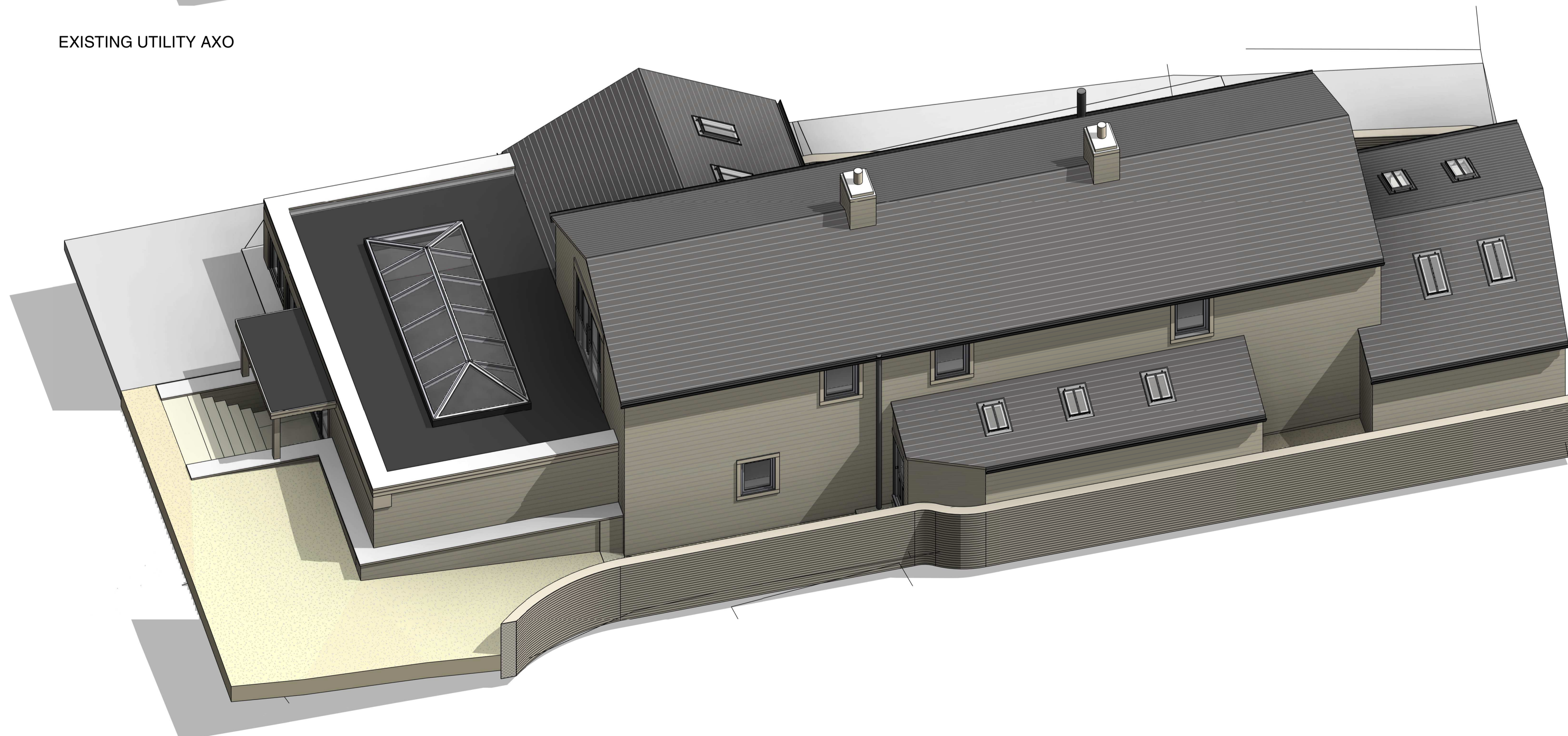
PROPOSED UTILITY AXO
