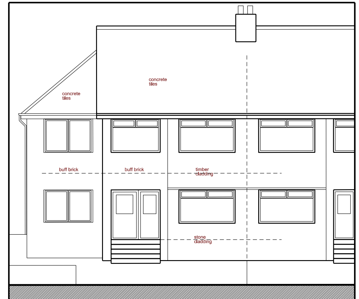
North Elevation - Proposed
