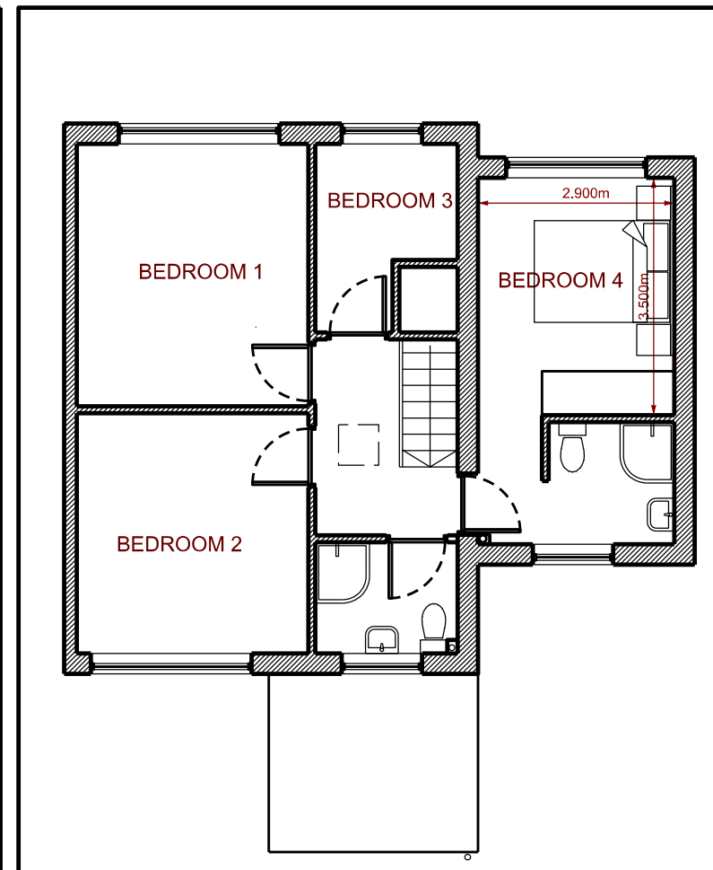
First Floor Plan - Proposed
