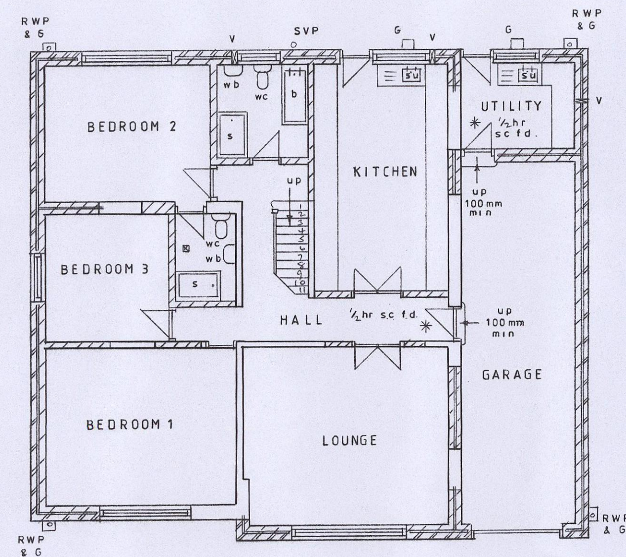
PROPOSED G.F. PLAN
