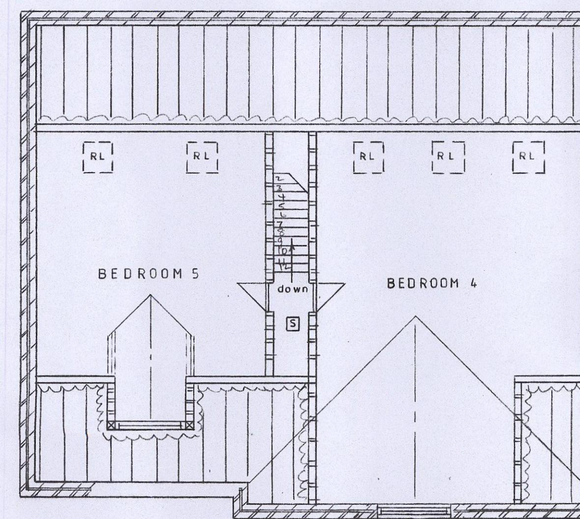
PROPOSED F.F. PLAN
