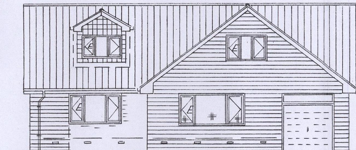
PROPOSED FRONT NORTH-EAST
