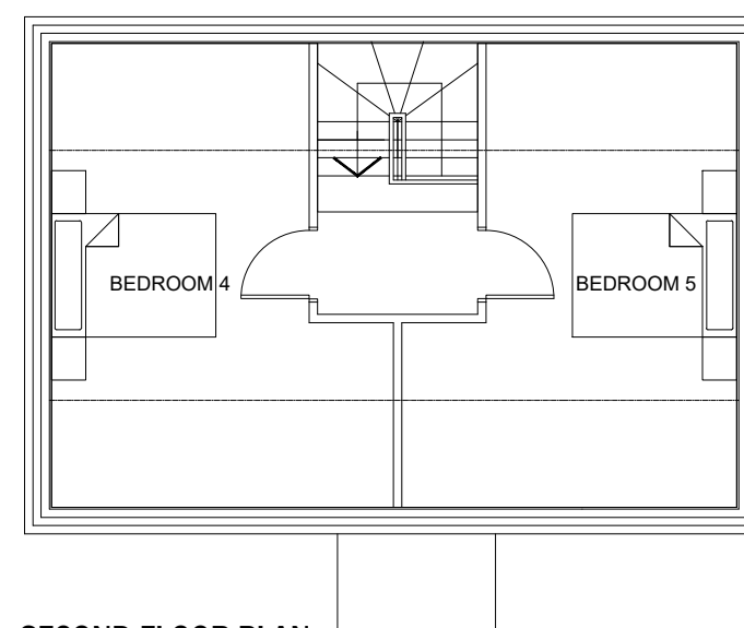
SECOND FLOOR PLAN AREA - 43.04sqm
