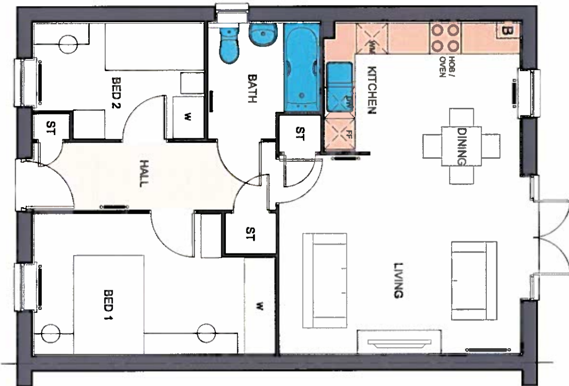
FLOOR PLAN
