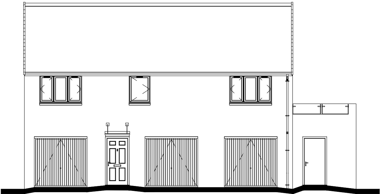
Front Elevation. 1 : 100
