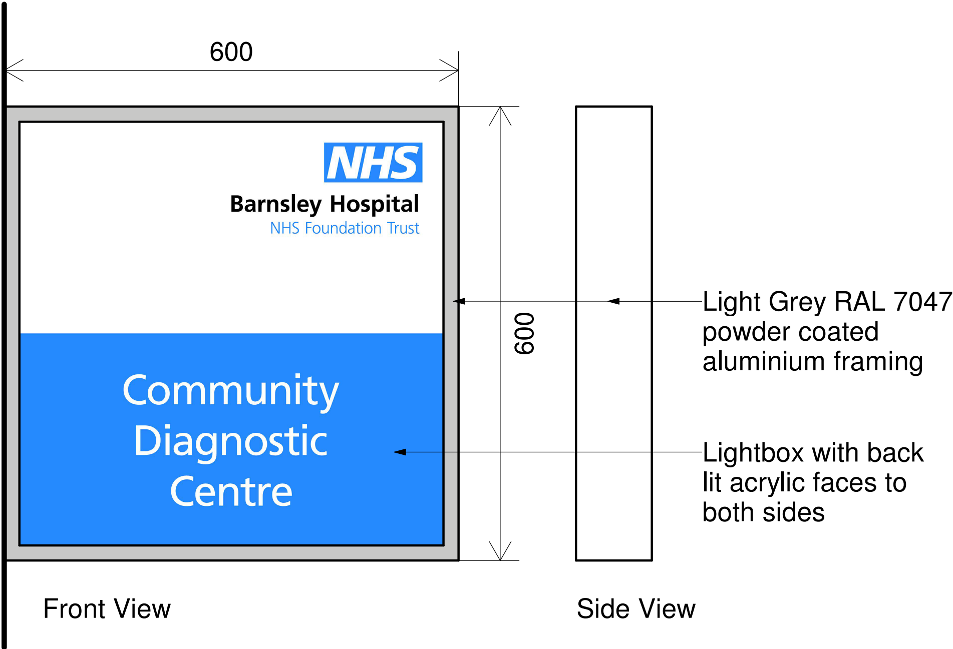
Proposed Illuminated Projected Sign 1 : 5 @ A1
