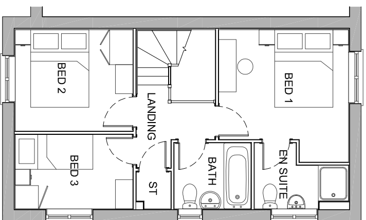
First Floor Layout
