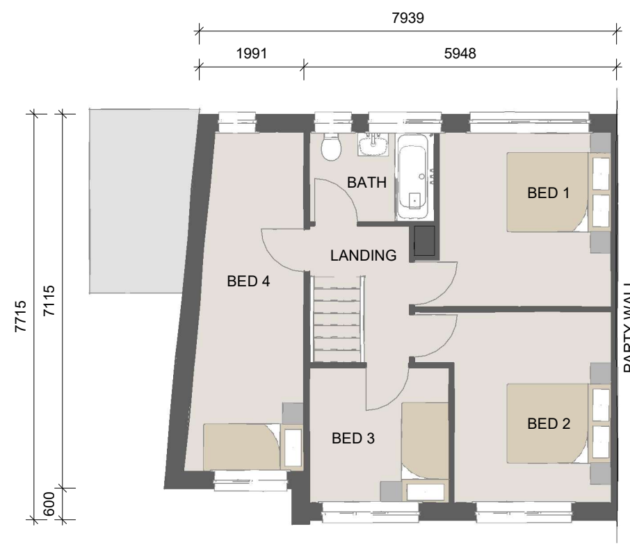
First Floor. 1 : 100
