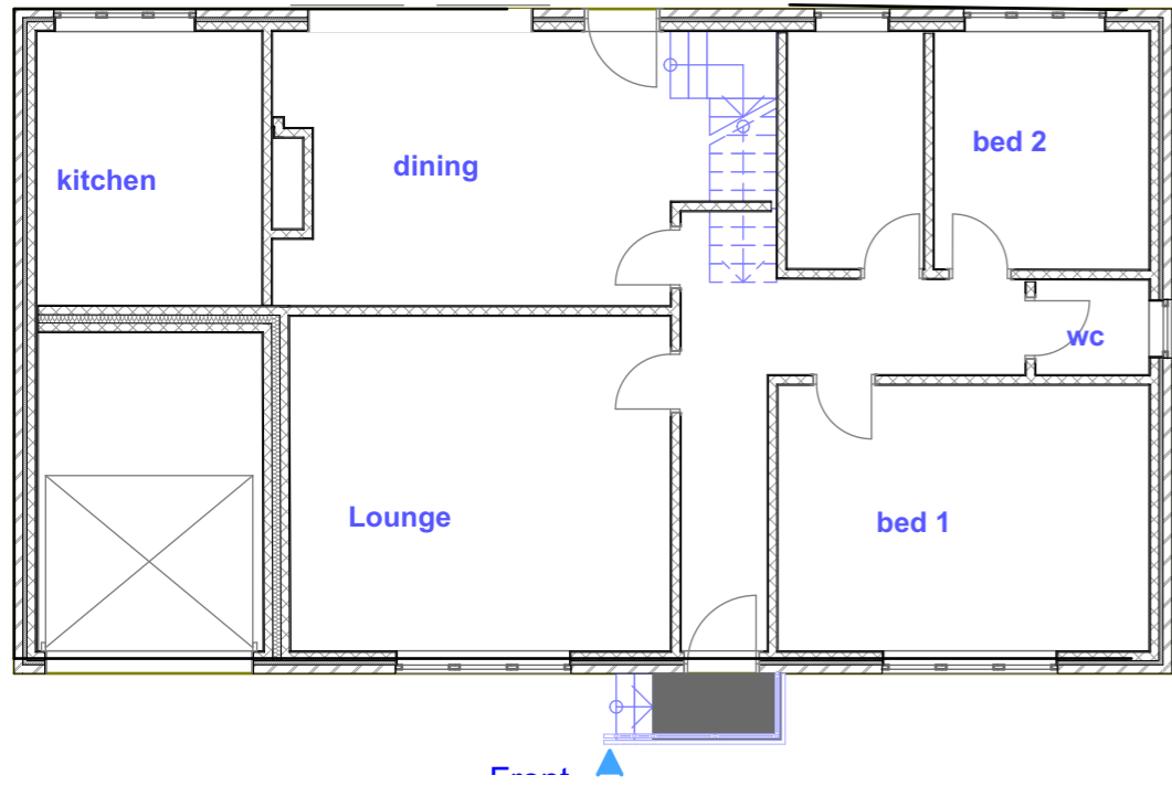
0. Ground Floor (1)
