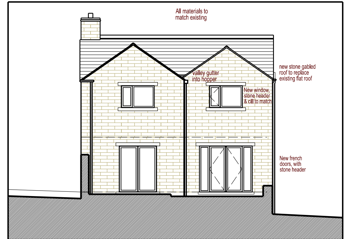
East Elevation
