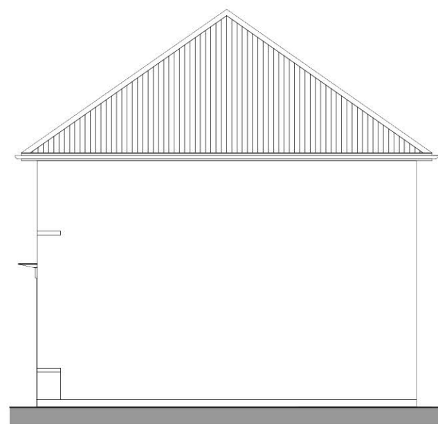
SIDE ELEVATION
